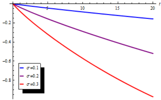
Figure 4: \text{Skew}(Y_t) with parametrization (5.10) using \sigma = 0.1 (blue), \sigma = 0.2 (purple) and \sigma = 0.3 (red).
