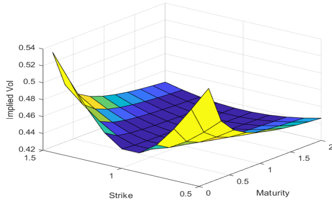
Figure 2: Normal implied volatility surface of the S^{R,1/2} model.
