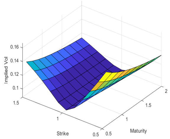
Figure 7: Implied volatility surface of the S^P model using b_H with H = 0.5 and \sigma = 0.05 .
