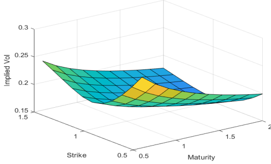
Figure 8: Implied volatility surface of the S^P model using b_H with H = 0.3 and \sigma = 0.1 .
