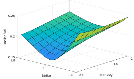
Figure 9: Implied volatility surface of the S^P model using b_H with H = 0.7 and \sigma = 0.1 .
