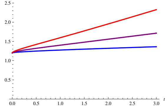
Figure 5: \text{Kurt}(Y_t) with parametrization (5.10) using \sigma = 0.1 (blue), \sigma = 0.2 (purple) and \sigma = 0.3 (red).
