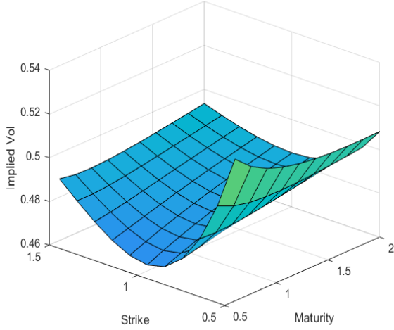
Figure 6: Implied volatility surface of the S^P model using b_H with H = 0.5 and \sigma = 0.25 .
