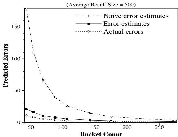
Figure 7: Quality Guarantees: Equality Predicates
