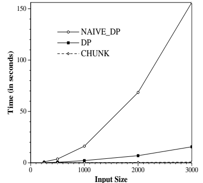
Figure 3: Running Times of Various Dynamic Programming-Based Algorithms
