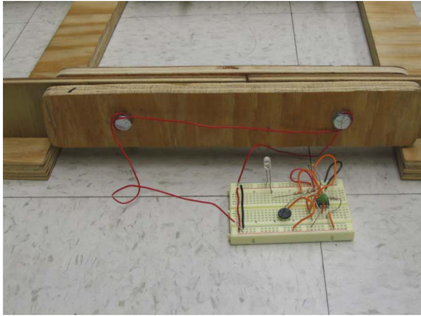
Side view of Track and IR circuit
