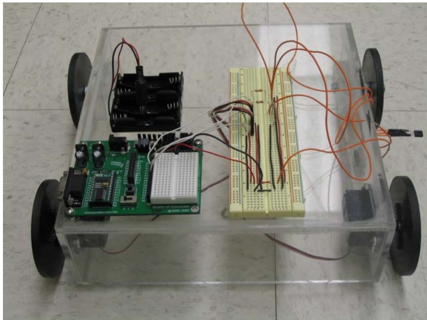
Top View
