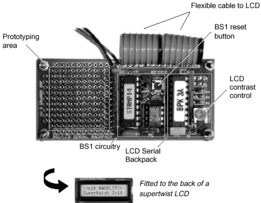
Figure 27.4: New kit combines BS1 and LCD in one package
