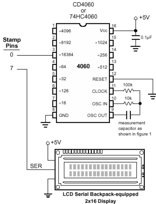
Figure 27.2: Schematic of H2O level test setup
