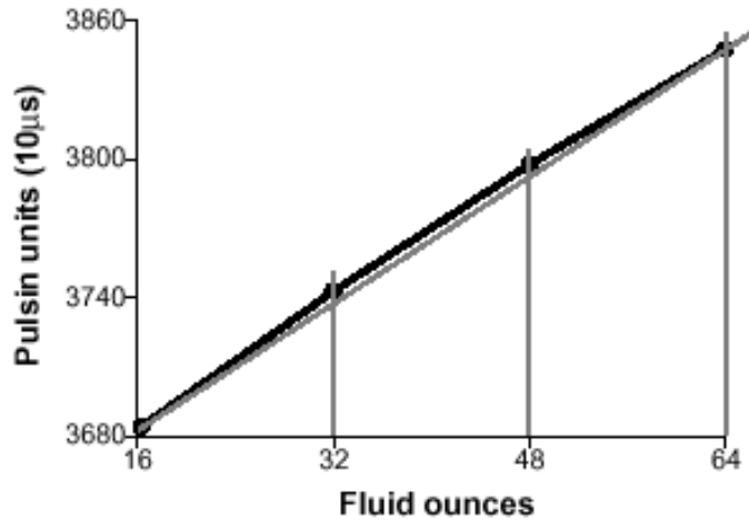
Figure 27.3: Graph of Pulsin versus water level.
