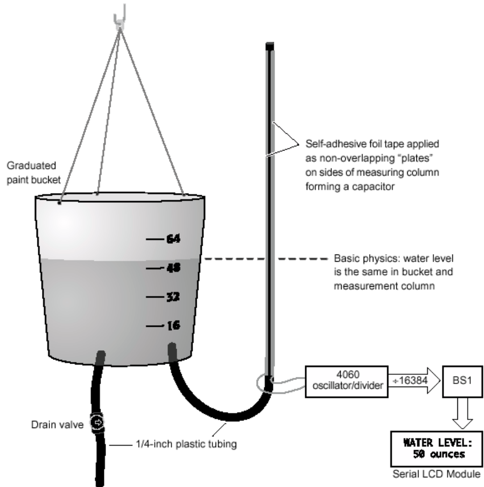
Figure 27.1: Water level test setup
